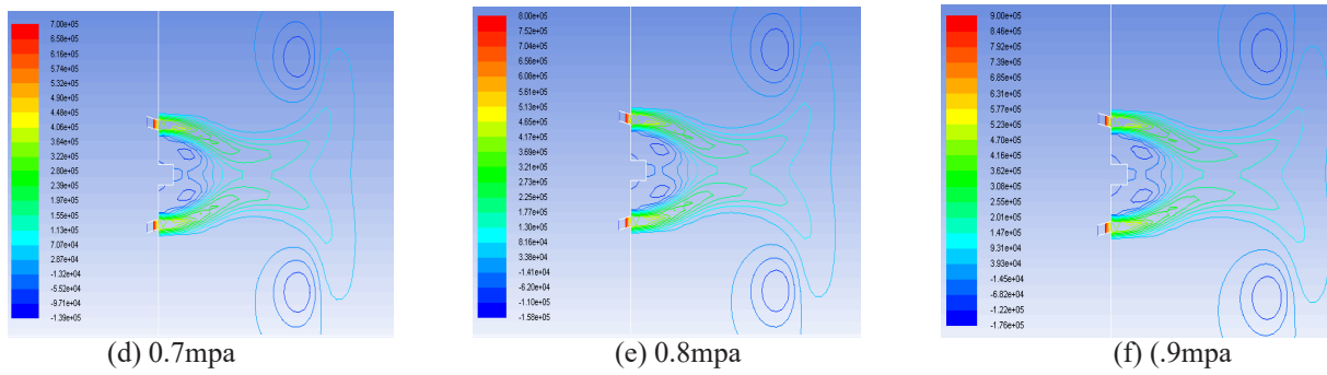
Figure 7. The pressure field of atomized gas under different gas pressures.
