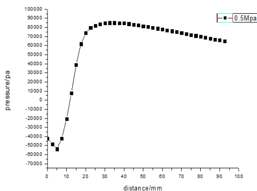
Figure 4. The pressure curve of atomized gas at the center axis of nozzle.
