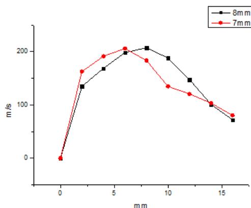
Figure 6. The relationship of air flow speed and distance at the front of liquid guide pipe.
