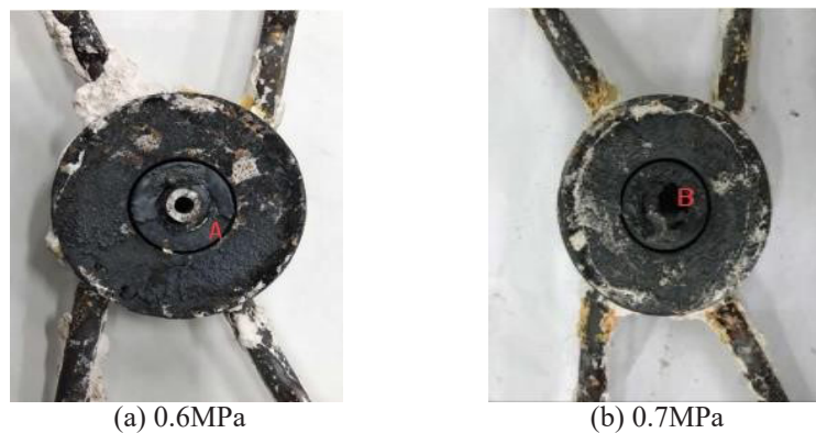
Figure 8. The adhesion at nozzle outlet under different atomization pressures.
