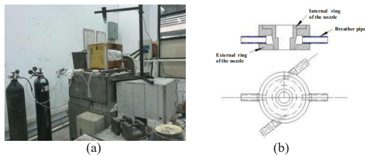
Figure 1. Self-made 10kg spray forming equipment and nozzle structure diagram. (a) Equipment; (b) Nozzle.
