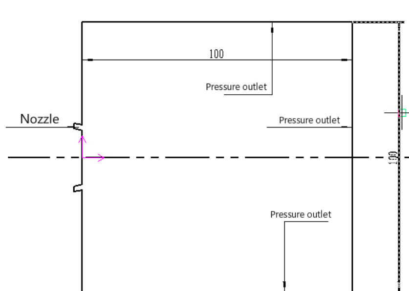
Figure 2. Physical model of flow field analysis for nozzle atomized gas.
