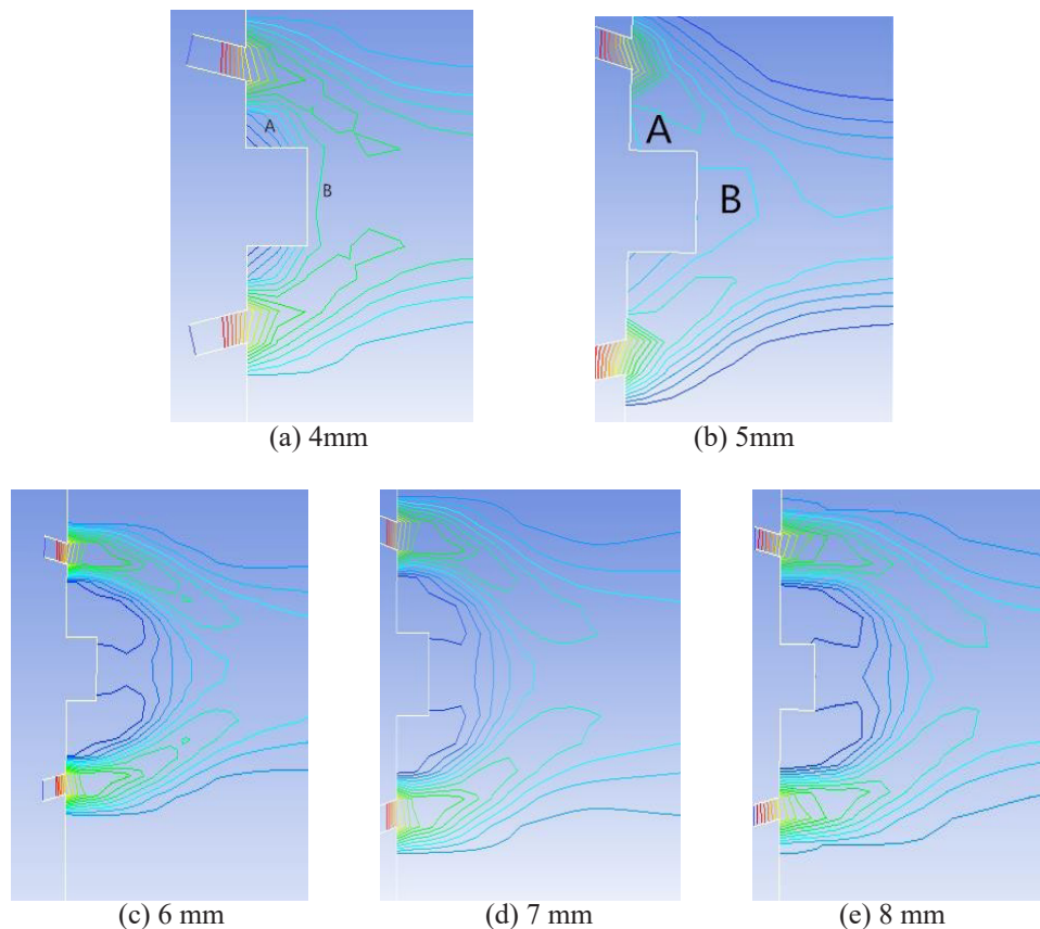
Figure 5. The distribution of atomized gas pressure field at different extension positions of liquid guide tube.
