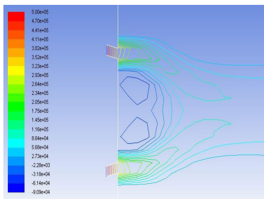
Figure 3. The contour map of pressure distribution for atomized gas flow field of nozzle.
