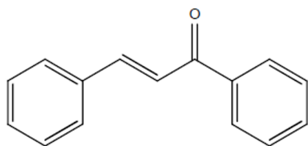
Figure 1. Chalcone structure
