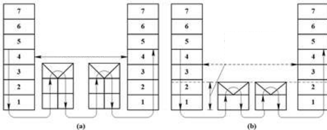
Figure 2.1: Compare X.25 networks and frame relay networks from the hierarchy
