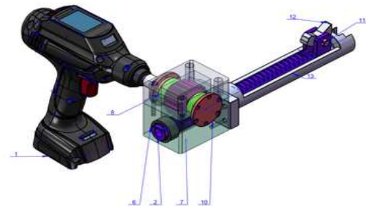
Fig.2 Model of Fast Lock Anchorage Tool
