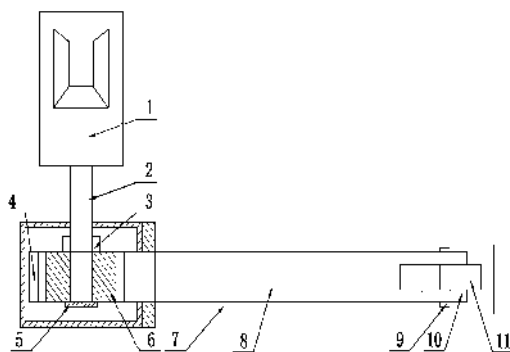
Fig.1 Schematic diagram of fast locking anchorage tool
